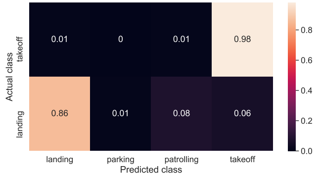
Fig. 5. Confusion matrix of trajectory classification.
