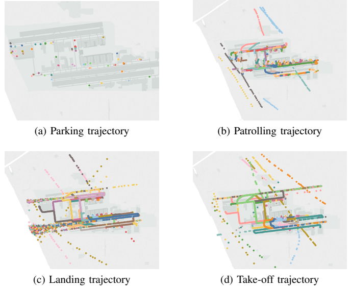
Fig. 4. Four classes of aircraft trajectories at airport from step 1.2 in data preprocessing.
