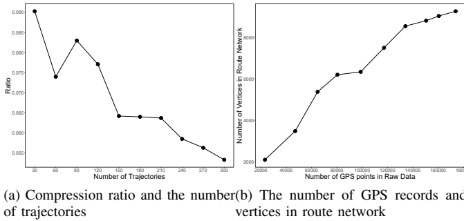
Fig. 6. Compression ratio.
